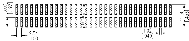
Recommended P.C.B Layout(Top Side) (PCB BOARD TOLERANCE±0.05)
