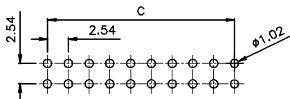
RECOMMEND PCB LAYOUT(TOLERANCE=±0.05)
