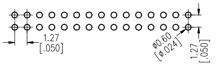
Recommended P.C.B Layout(Top Side) (PCB BOARD TOLERANCE ±0.05)
