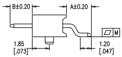
TYPE-2: W/T POST
